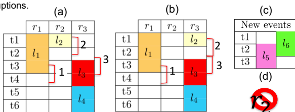
Fig2: Two optimal timetables in terms of compactness, and two possible disruptions. r1 to r3 are rooms, t1 to t6 are time slots and l1 to l6 are events. The timetable (a) is better for the disruption (c) and the timetable (b) is better for the disruption (d).
